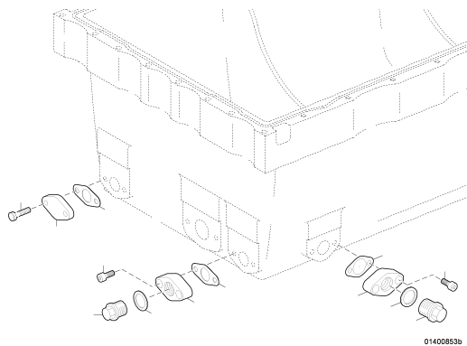
FLANGE OILPAN 7 SOLID 3 W/M30 HOLE+PLUGS UPC.06E02 0011
