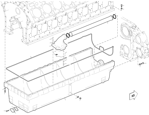
PAN OIL GENSET GRAY CAST IRON X00025458 UPC.06E00 1009
